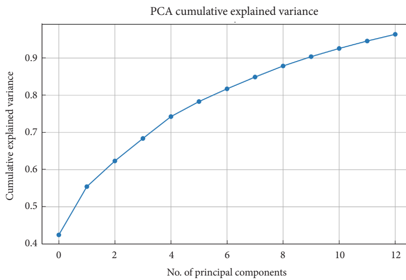
Supplementary Fig. 2. Principal component analysis (PCA) cumulative explained variance plot. The x -axis represents the number of principal components, while the y -axis indicates the cumulative explained variance.
