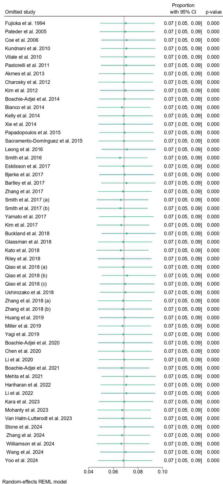
Supplementary Fig. 10. Leave-one-out analysis. CI, confidence interval; REML, restricted maximum likelihood.
